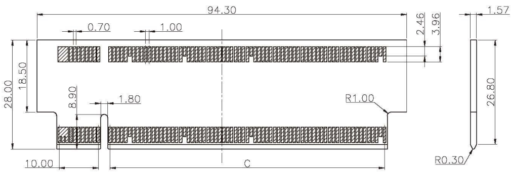
RECOMMENDED MODULE LAYOUT
